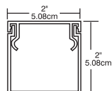
Raceway 2 x 2
