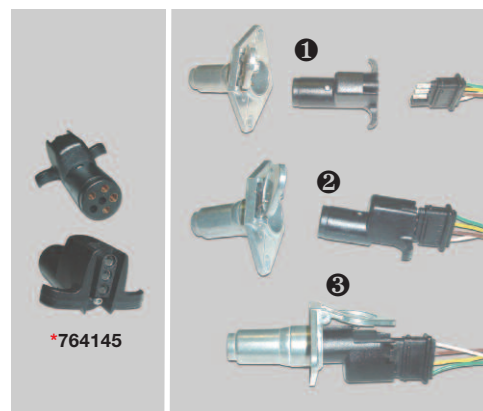
6-Pole to 4-Pole RV Connector Adapter
