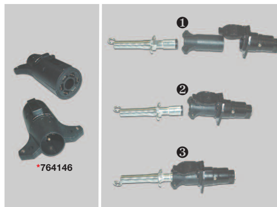
7-Pole to 6-Pole RV Connector Adapter
