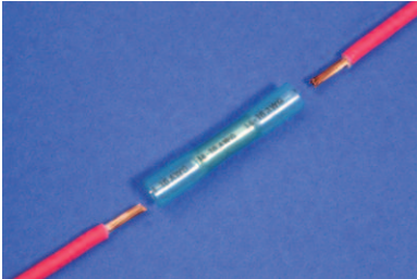
1. Strip Connector Wire
