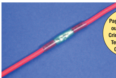
5. Completed Waterproof Connection
