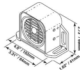
Light Duty Back-up Alarm
