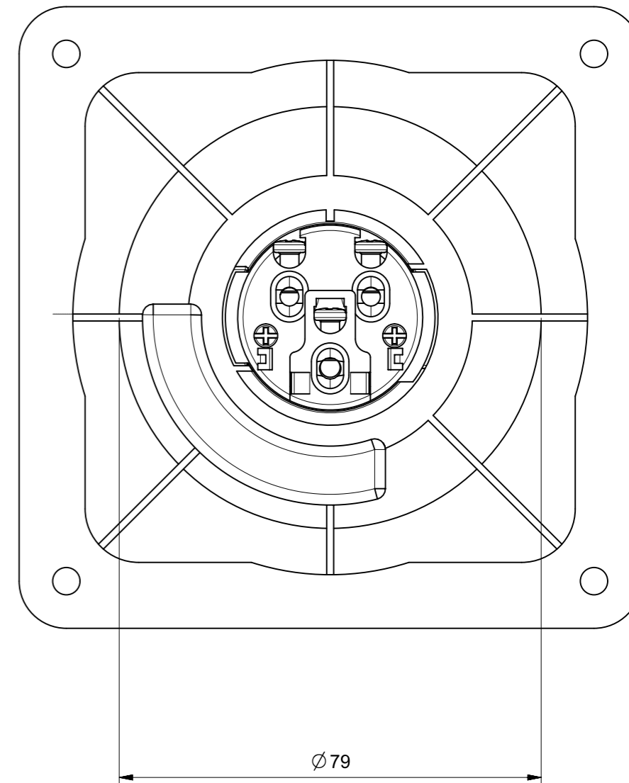
FORATURA PANNELLO // PANEL DRILLING HOLE
